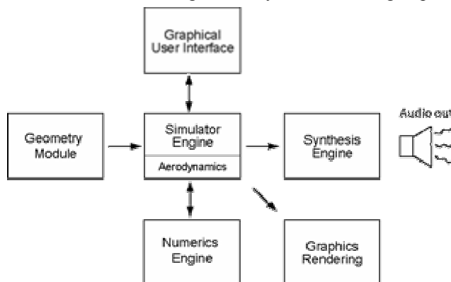
Figure 2: Block diagram of ArtSS proposed design.
